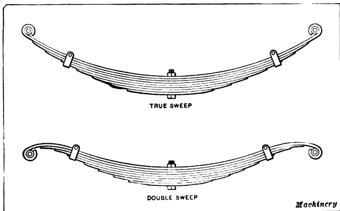
Fig. 2—General arrangement of spring plates, clips, etc., in true and double sweep springs
